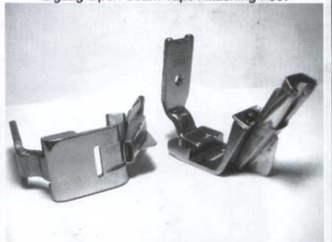
人字開式縫面貼壓腳 Zigzag Open Seam Tape Attaching Foot
